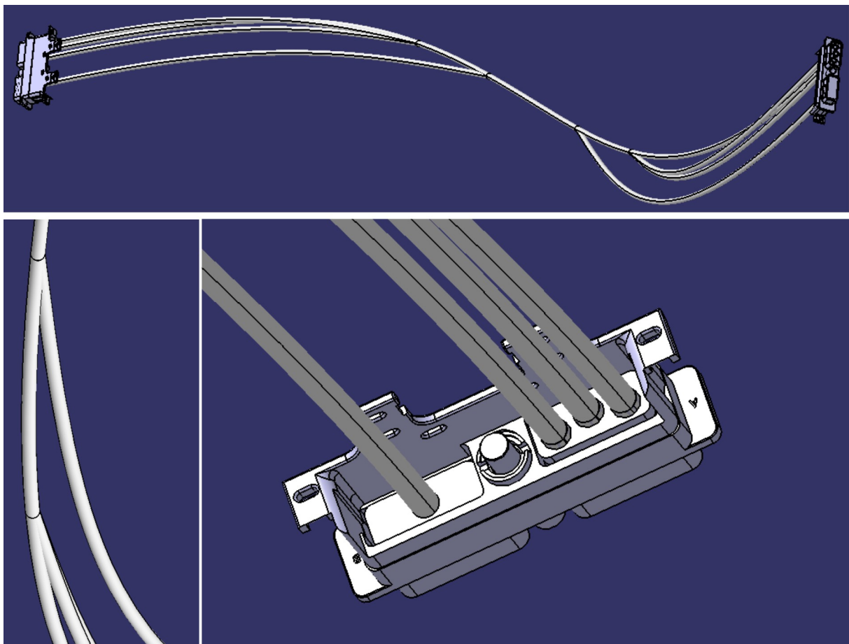
Figure 19: 3D Representation
