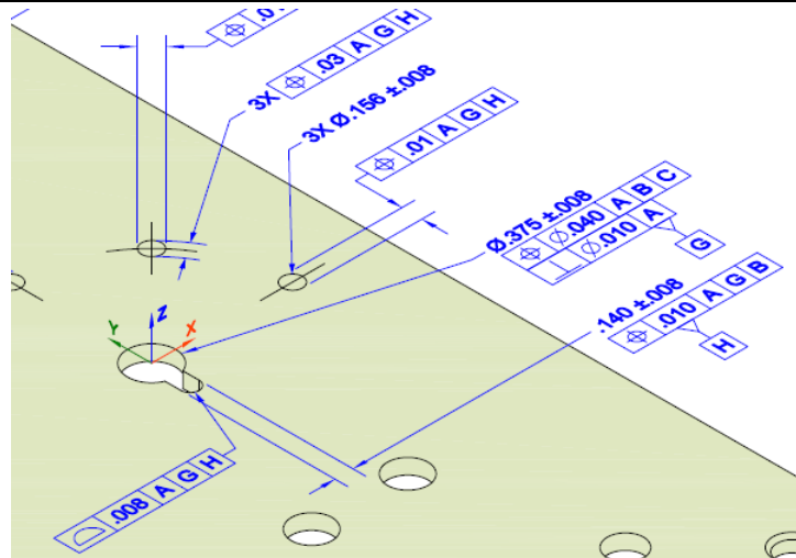
Figure 10: NIST Test Case FTC09, View C, Detail of Slotted Hole
