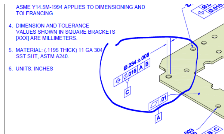
Figure 9: NIST Test Case FTC09, View A, Detail of Hole
