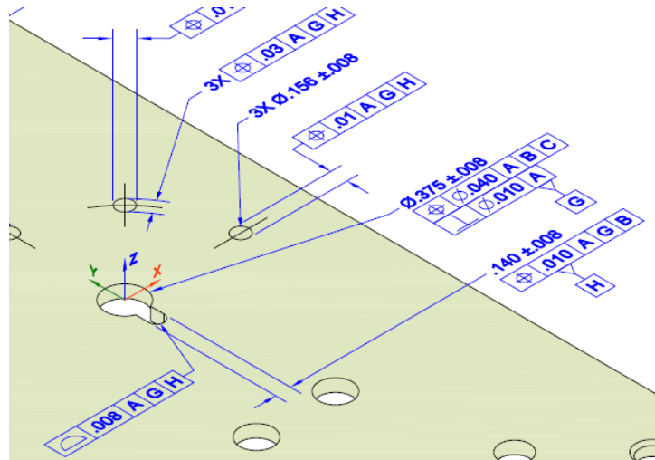
Figure 7: NIST Test Case FTC09, View C, Detail of Slotted Hole
