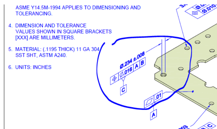
Figure 6: NIST Test Case FTC09, View A, Detail of Hole
