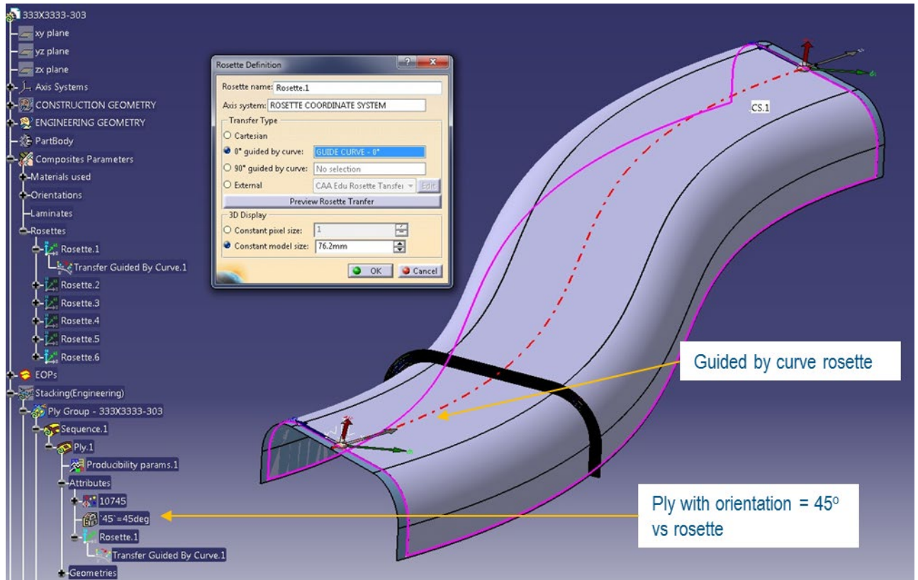
Figure 9: ASME_Y14.37_RosetteType2.CATPart
