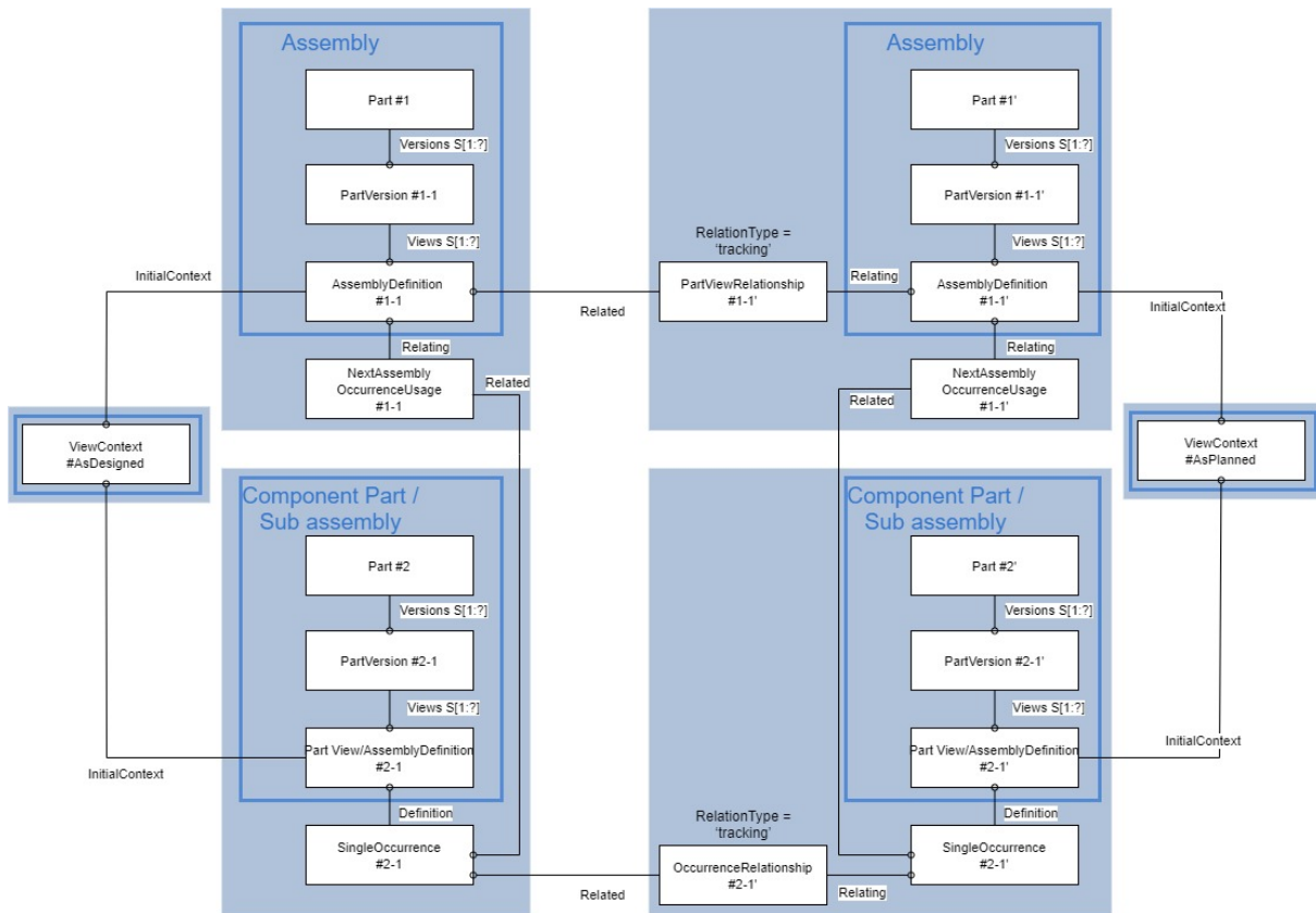
Figure 75 Representation of tracking relationship
