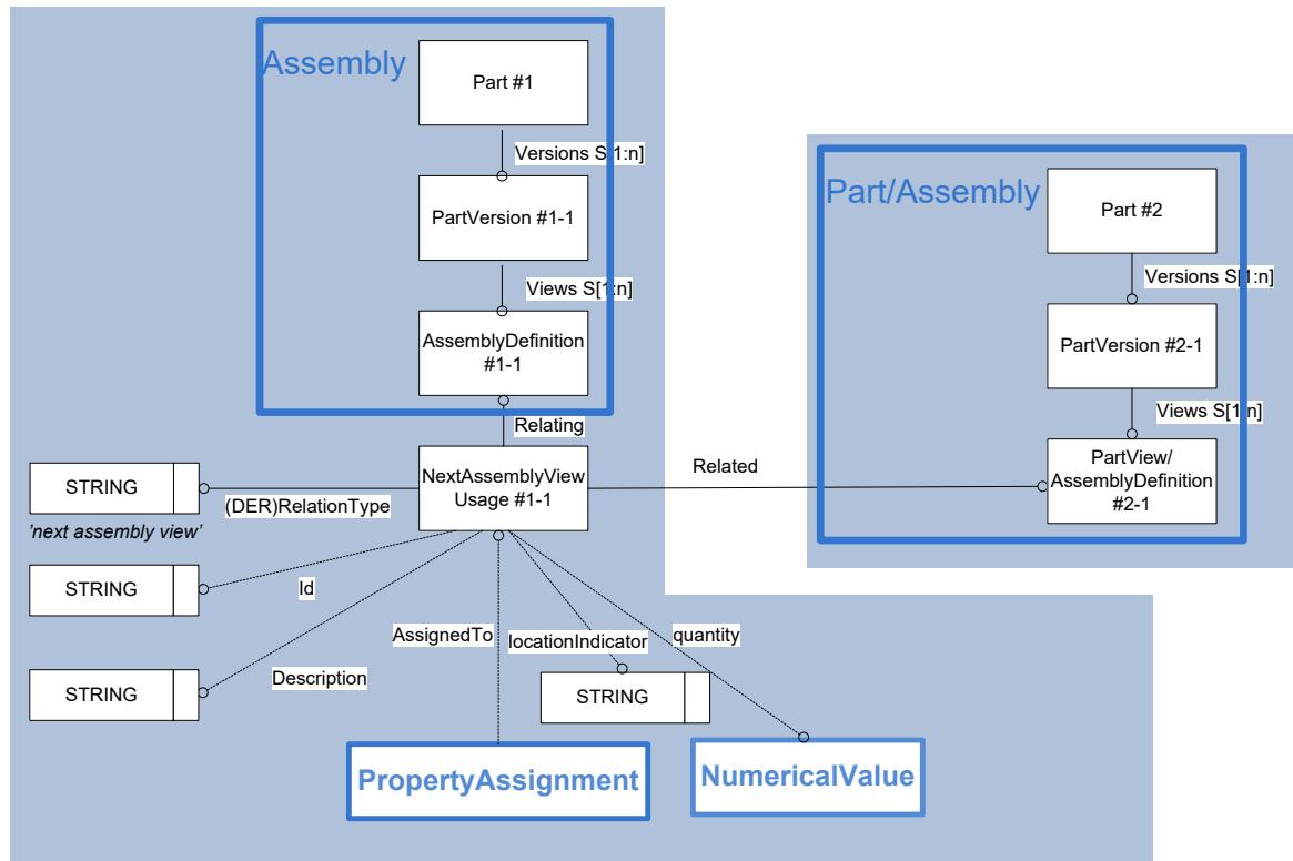
Figure 32: Template "PartViewRelationship" for quantity (+ properties)
