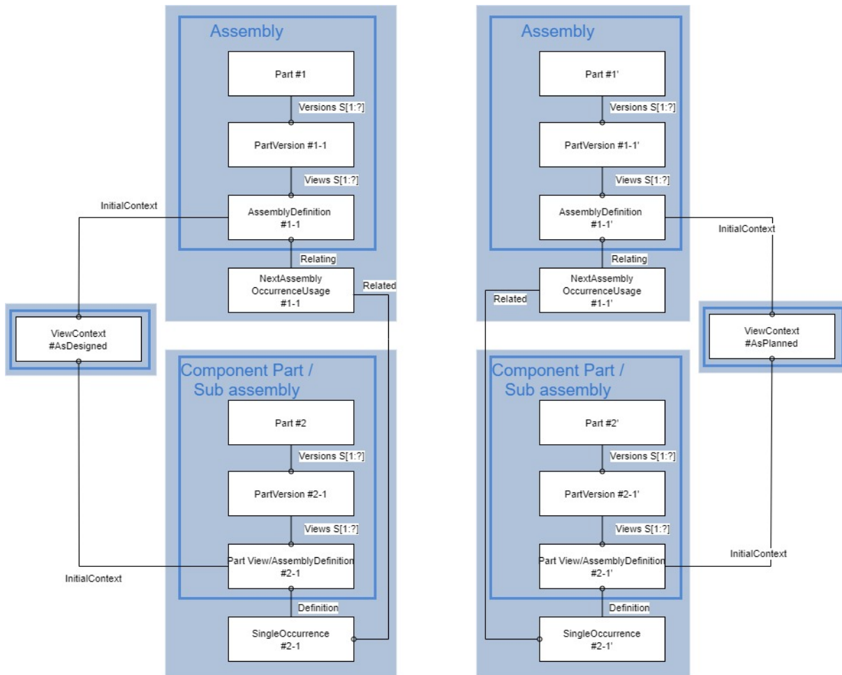
Figure 74 Representation of As Designed and As Planned views
