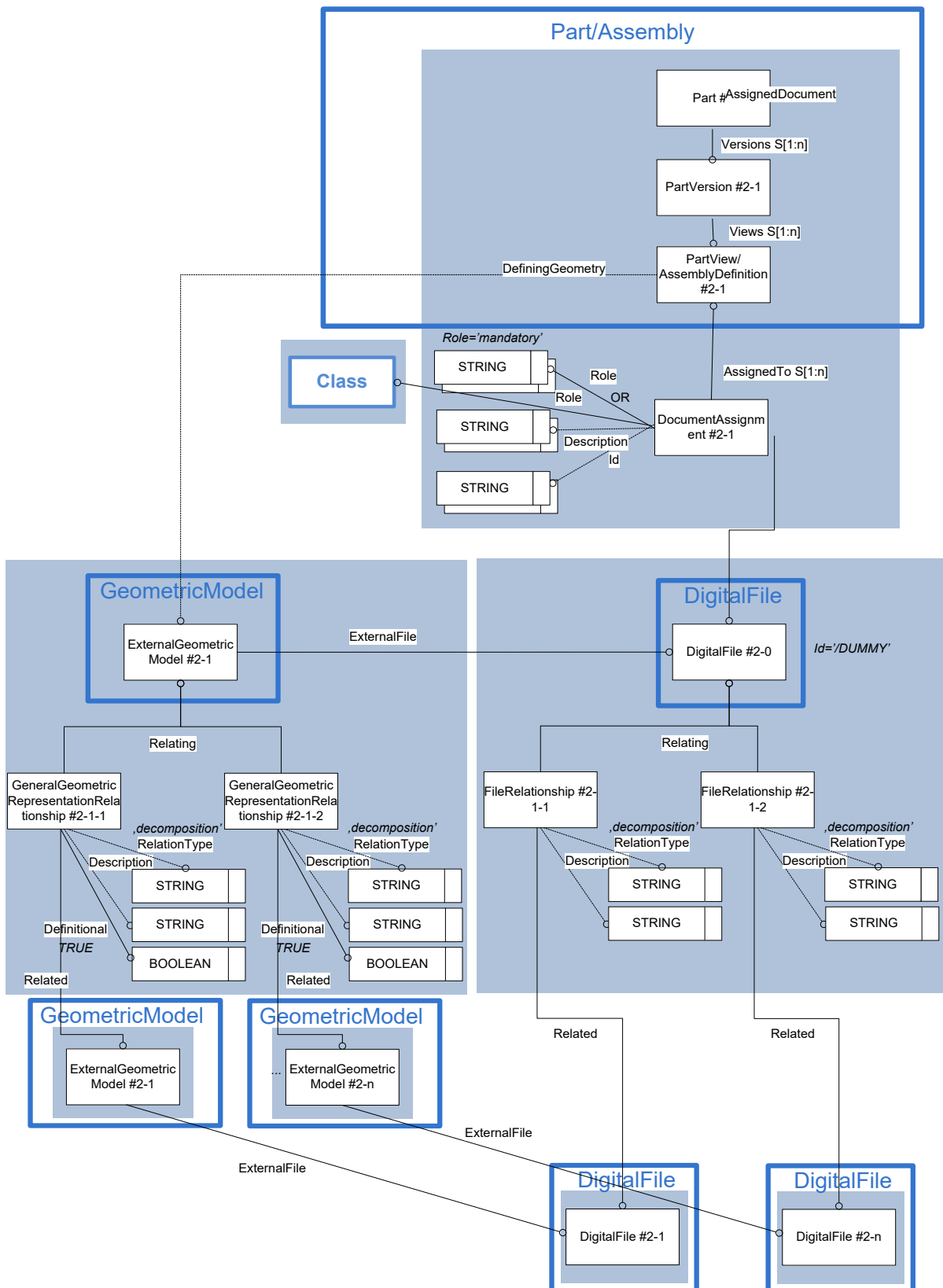
Figure 53: Model splitting for "CAX Representation for DocumentAssignment"
